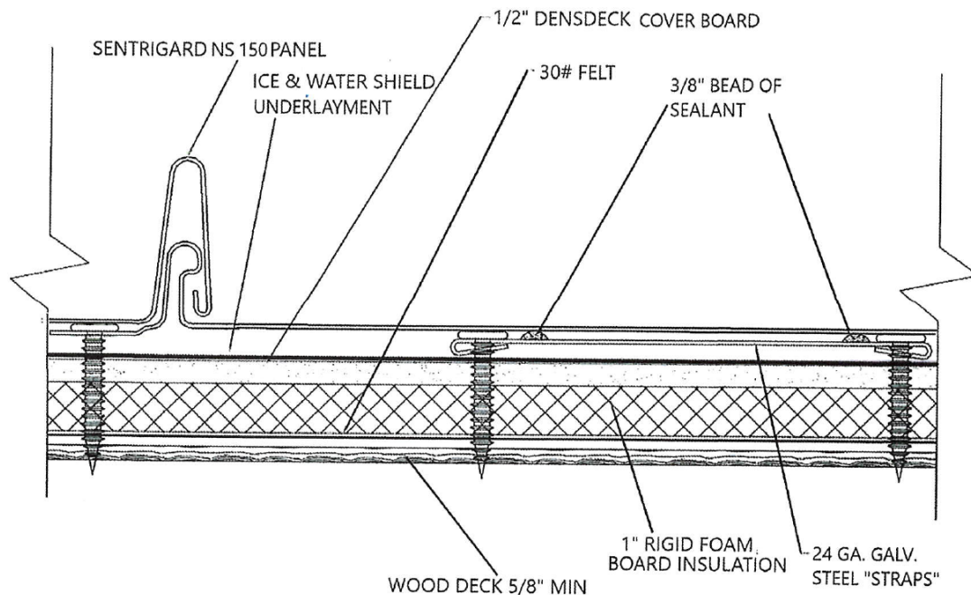
Typical Panel Assembly View (Method 2)
