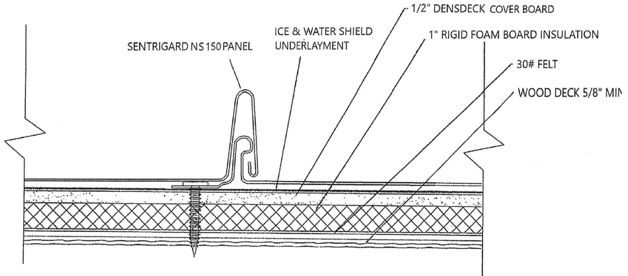
Typical Panel Assembly View (Method 1 )
